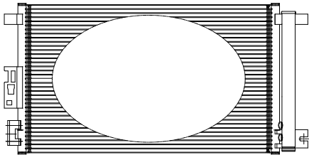
693(L)x358(W)x18(T)
