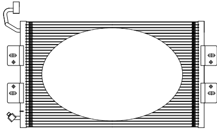
671(L)x367(W)x18(T)
