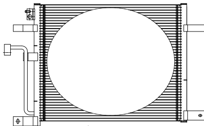
550(L)x437(W)x18(T)
