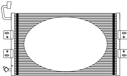
671(L)x367(W)x18(T)
