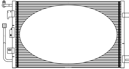
698(L)x397(W)x18(T)
