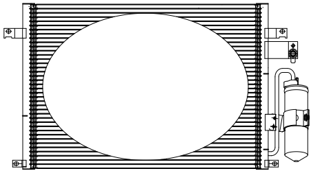
632(L)x358(W)x18(T)
