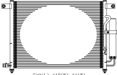
582(L)x417(W)x18(T)
