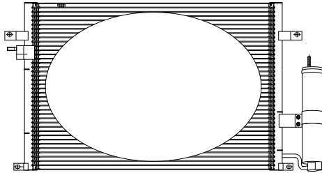
642(L)x387(W)x18(T)
