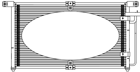
693(L)x374(W)x18(T)
