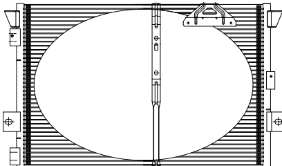
742(L)x339(W)x18(T)
