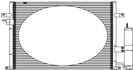
642(L)x387(W)x18(T)
